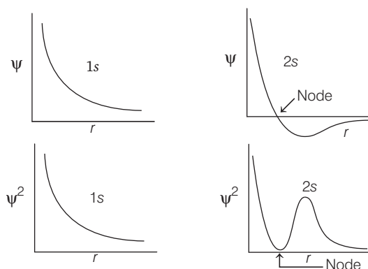
Plot of \psi and \psi^2 for 1s and 2s orbitals
