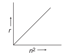
Variation of r with n^2
